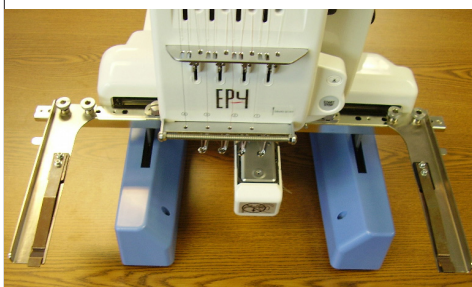
Center Position for Melco Hoop Arms
