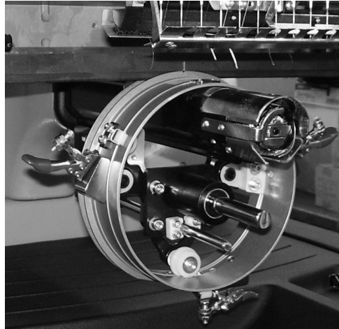
Picture 1: AMAYA XT with XT WACF Driver (note that the top 2 Locking Clamps are in the open position)
